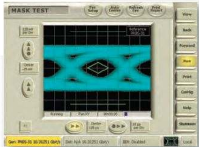
XFI compliant electrical stressed eye
